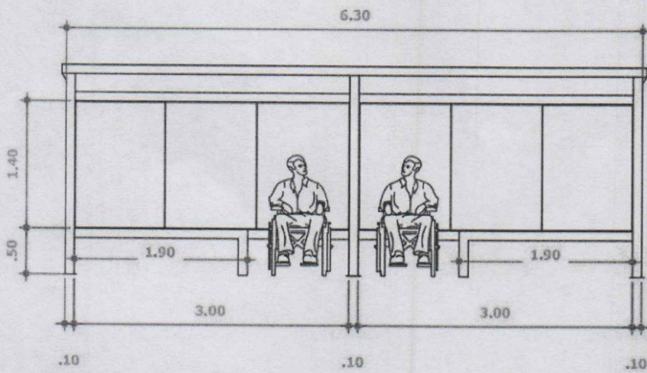
VISTA FRONTAL
