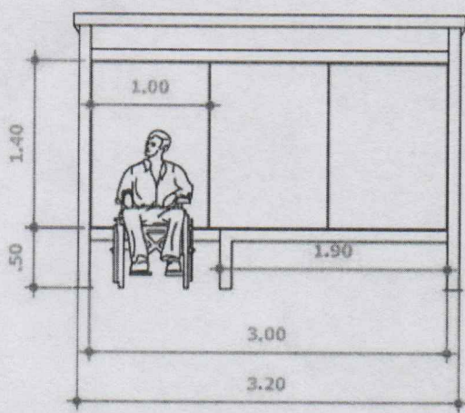
VISTA FRONTAL
